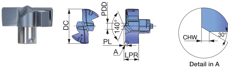
Detail in A
